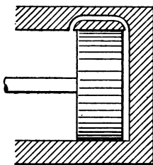
FIG. 39.—Uncovering port to release clearance pressure.
